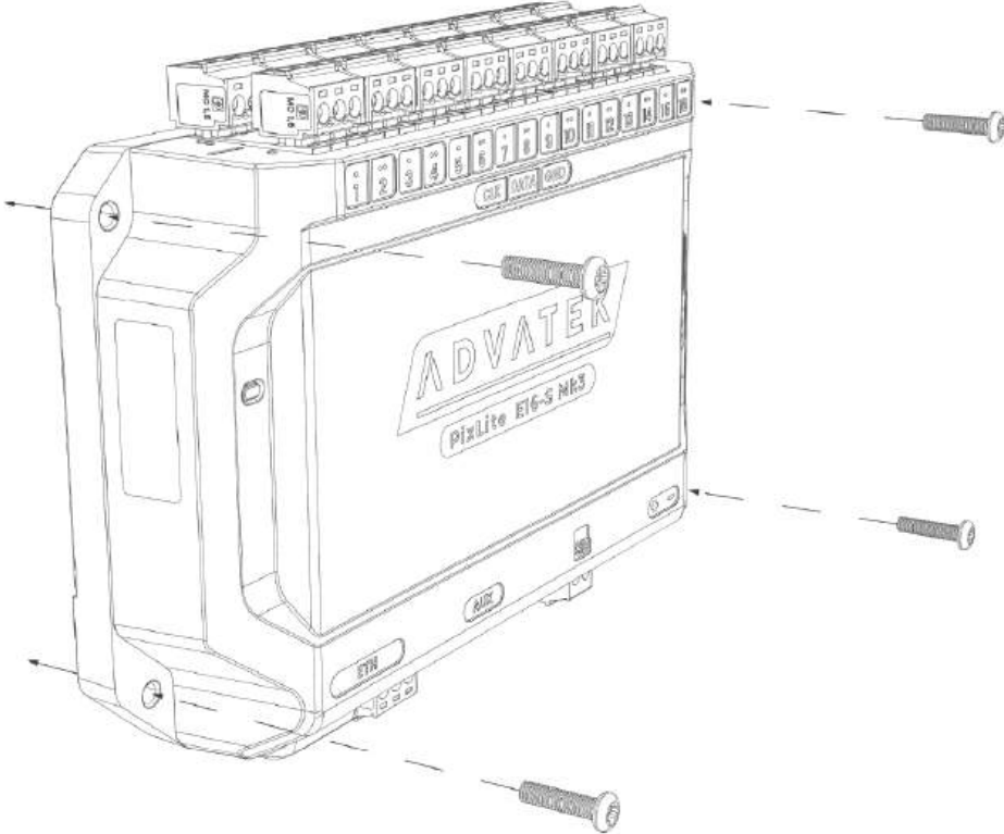
Figure 2: Controller Assembled to Flat Surface
