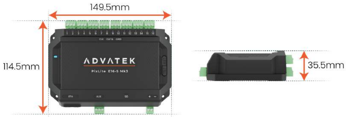
Figure 16: Mechanical Specifications
