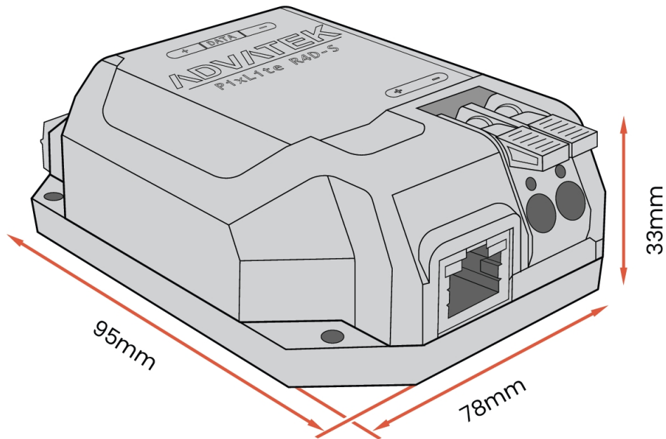
Figure 12: Receiver Mechanical Specifications
