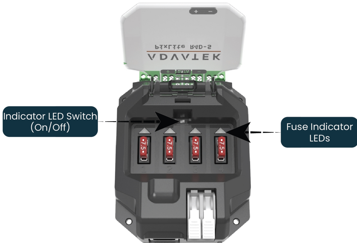
Figure 11: Position of Indicator LEDs and Switch
