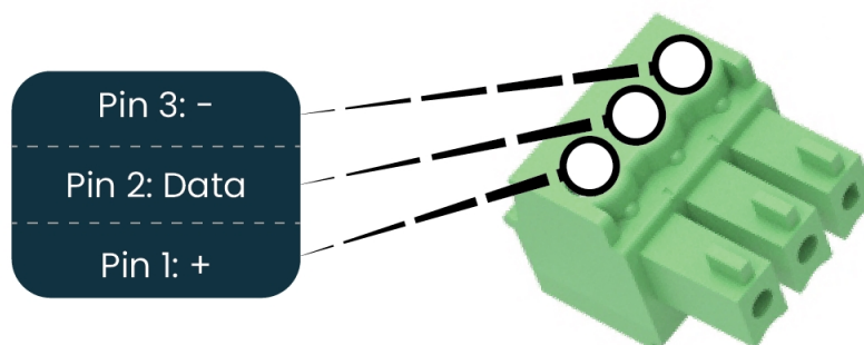
Figure 9: Pixel Output Pinout
