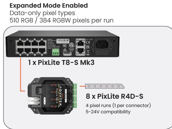
Figure 8: Connecting Receivers to Transmitter
